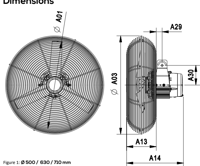
Figure 1: Ø 500 / 630 / 710 mm
